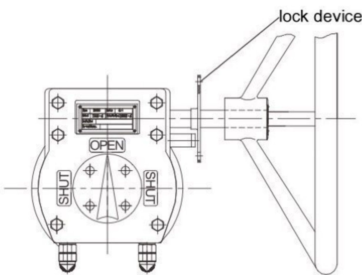
Gear Operation (Optional) SIZE : NPS 2 \frac{1}{2} ~ NPS 8
