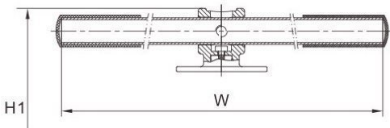
Gear Operation (Optional) SIZE : NPS 2 \frac{1}{2} ~ NPS 8
